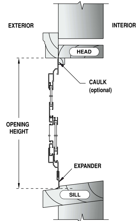
FIGURE 2: SIDE VIEW VERTICAL SECTION (Model L201 shown)
